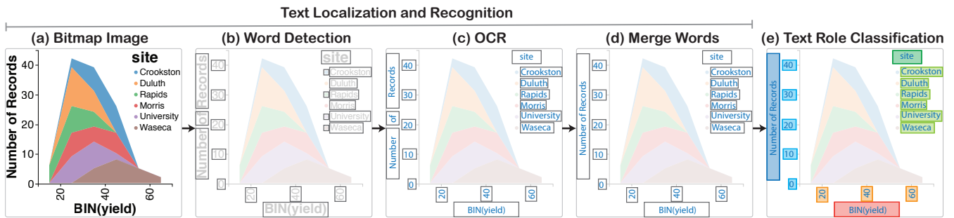
Figure 4: Text analysis pipeline. (a) Initial bitmap image. (b) Identify bounding boxes for words; note that some boxes are incorrect. (c) Use OCR to recover text for each box. (d) Merge words in lines. (e) Use geometric features of bounding boxes to classify their role in the chart.
