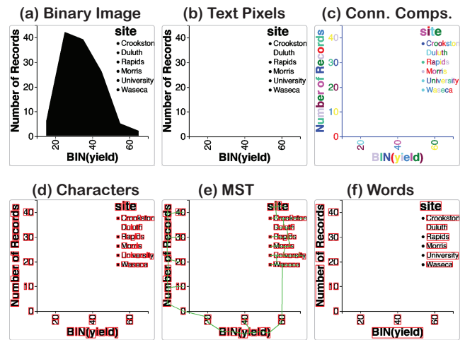
Figure 5: Word detection process. (a) Initial binarized image. (b) Clean image with non-text pixels removed. (c) Connected components. (d) Filter region candidates using geometric properties. (e) Minimal Spanning Tree using boxes as vertices and distances as edges weights. (f) Detected words after pruning edges in the MST.
